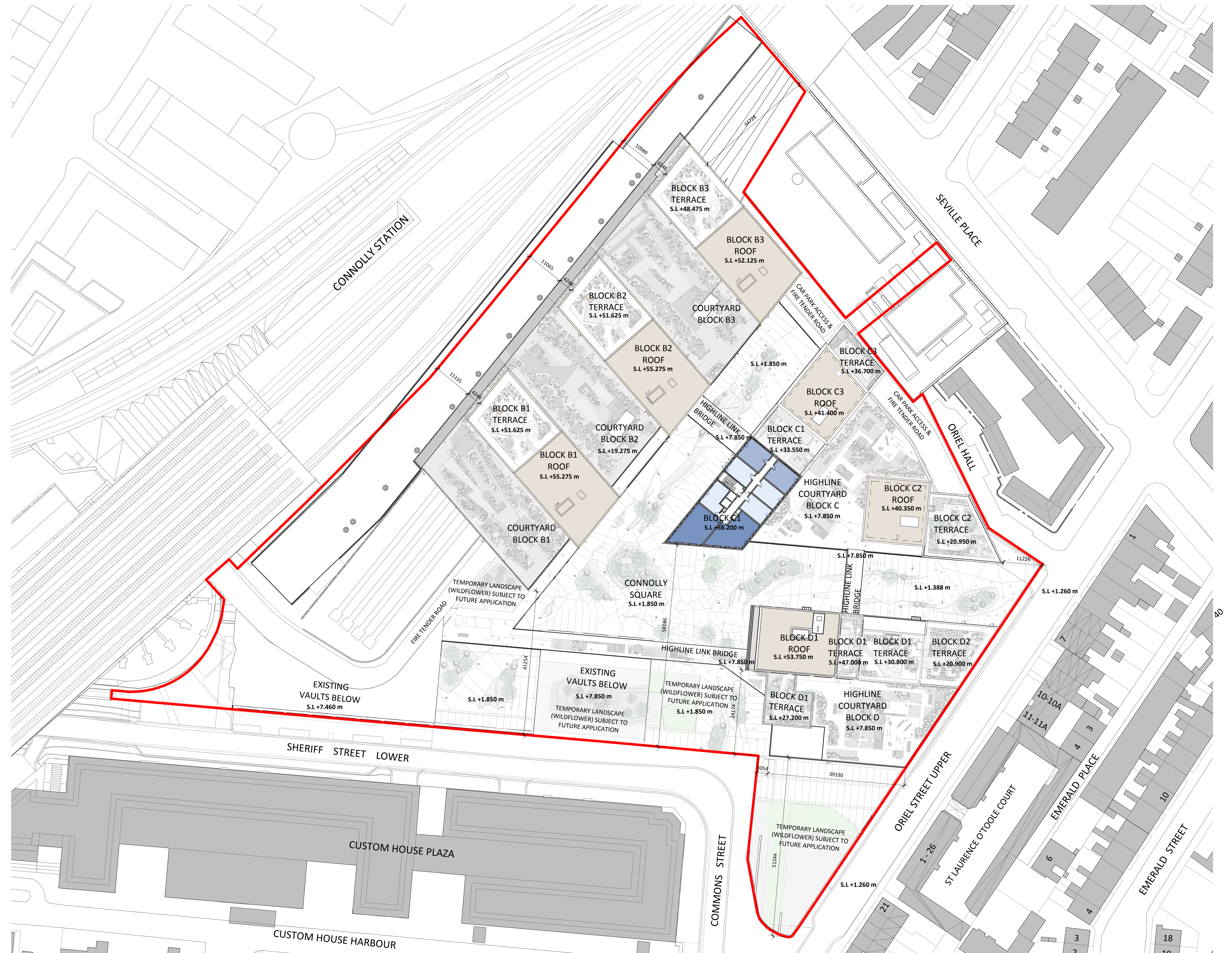
1 SITE LAYOUT PLAN - LEVEL 20 1:500
